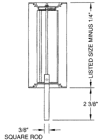
MODEL - OBD-RD-DM - ROD OPERATOR
