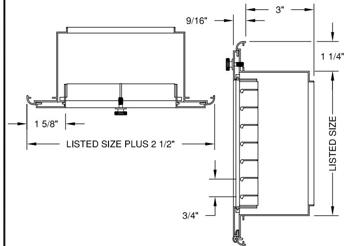
MODEL - GFXFS - 2" FILTER RACK
