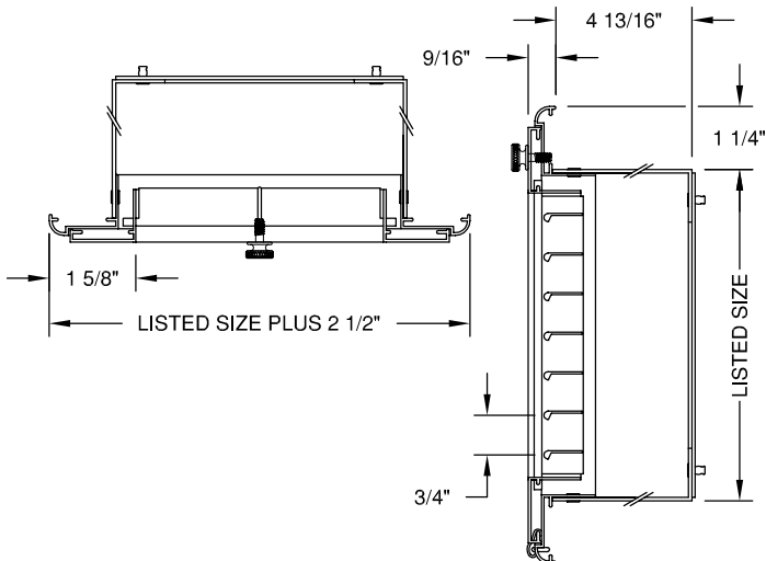
MODEL - GFXFS- 4" FILTER RACK
