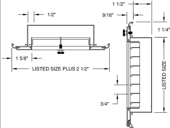
MODEL - GFXFS - 1" FILTER RACK
