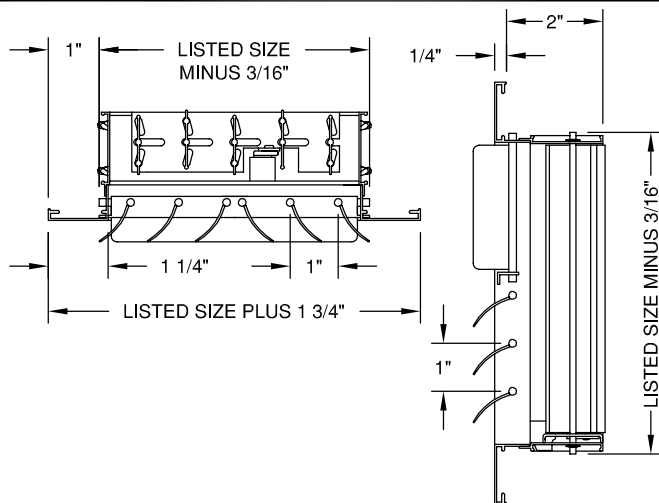
MODEL - C3244O - OPPOSED BLADE DAMPER
