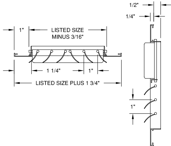
MODEL - C3244 - GRILLE
