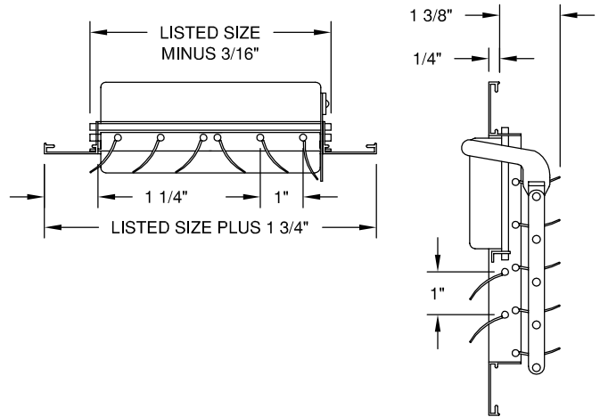
MODEL - C3244M - MULTI-SHUTTER DAMPER
