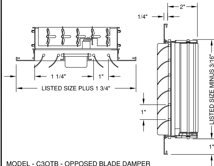
MODEL - C3OTB - OPPOSED BLADE DAMPER
