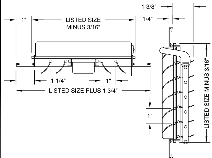
MODEL - C3MTB - MULTI-SHUTTER DAMPER
