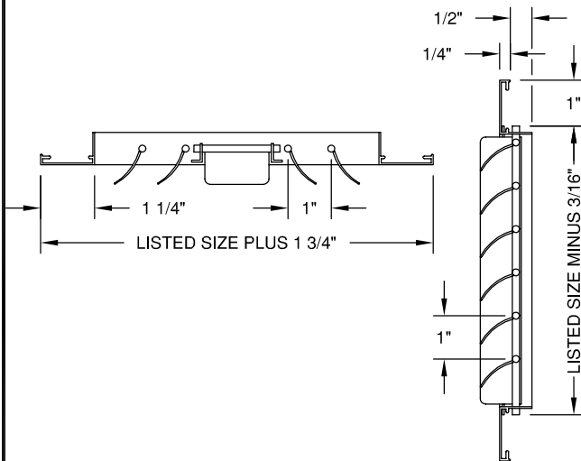
MODEL - C3TB - 3 WAY TEE BAR - GRILLE
