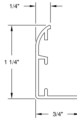
MODEL - C2BLM - MULTI-SHUTTER DAMPER
