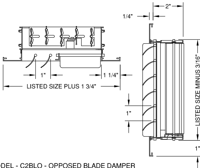
MODEL - C2BLO - OPPOSED BLADE DAMPER
