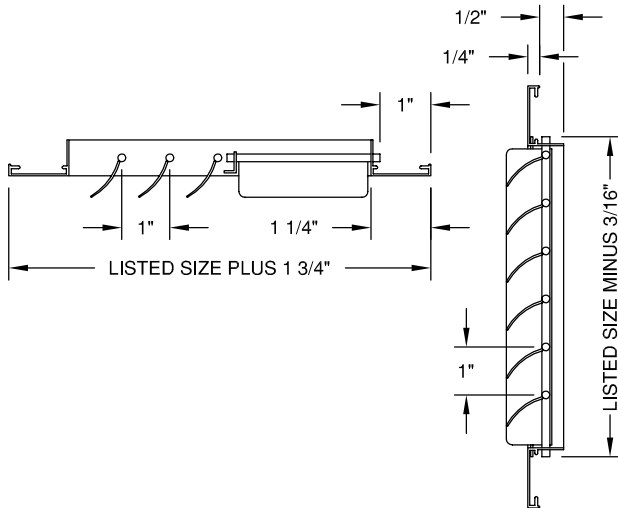
MODEL - C2BL - GRILLE
