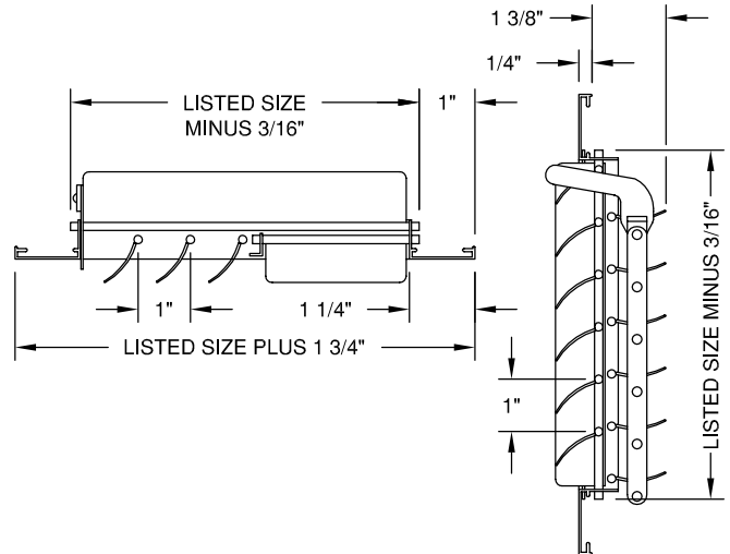
MODEL - C2BLM - MULTI-SHUTTER DAMPER
