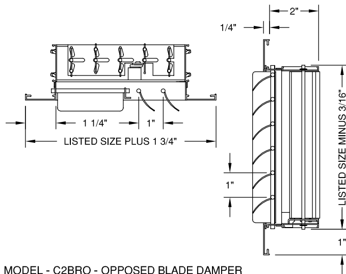
MODEL - C2BRO - OPPOSED BLADE DAMPER
