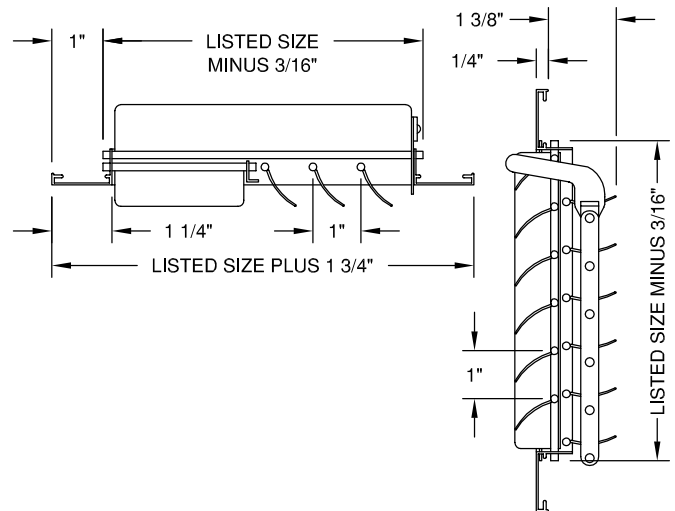
MODEL - C2BRM - MULTI-SHUTTER DAMPER
