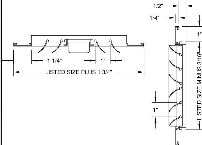
MODEL - C4 - GRILLE
