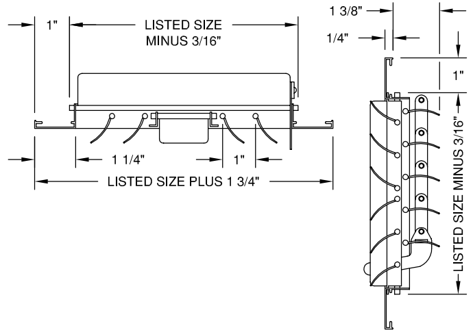
MODEL - C4M - MULTI-SHUTTER DAMPER
