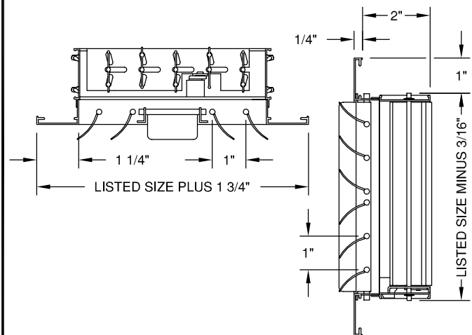
MODEL - C4O - OPPOSED BLADE DAMPER
