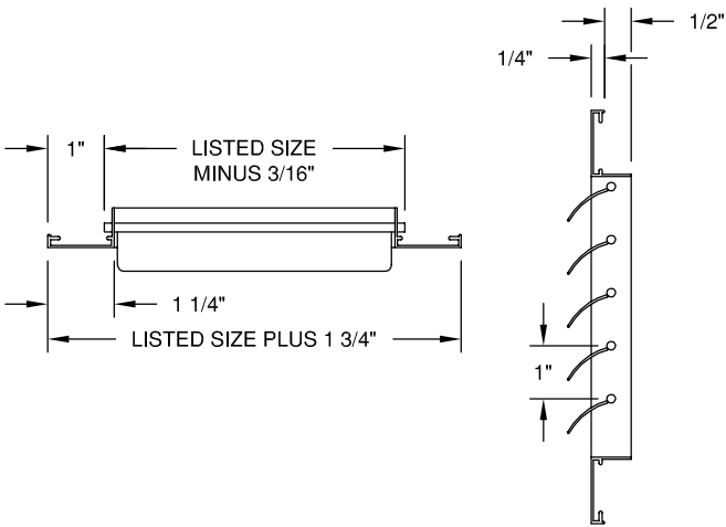
MODEL - C1L - 1 WAY LONG - GRILLE
