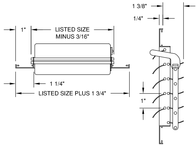
MODEL - C1LM - 1 WAY LONG - MULTI-SHUTTER DAMPER
