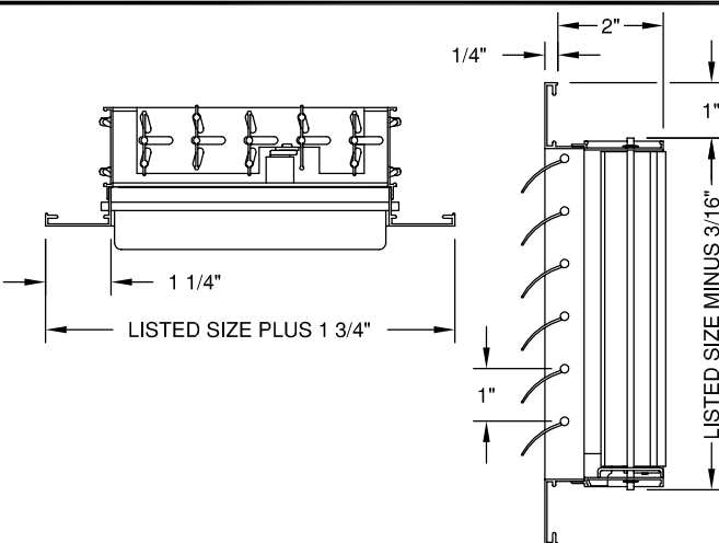
MODEL - C1LO - 1 WAY LONG - OPPOSED BLADE DAMPER
